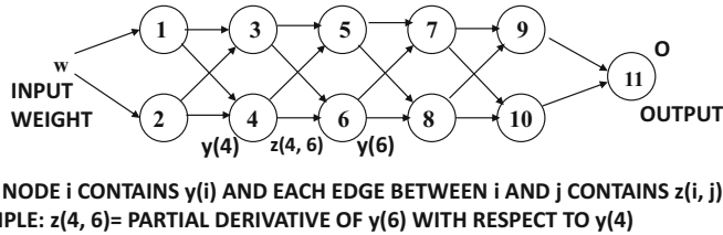
Figure 3.5: Example of computational graph with edges corresponding to local partial derivatives
