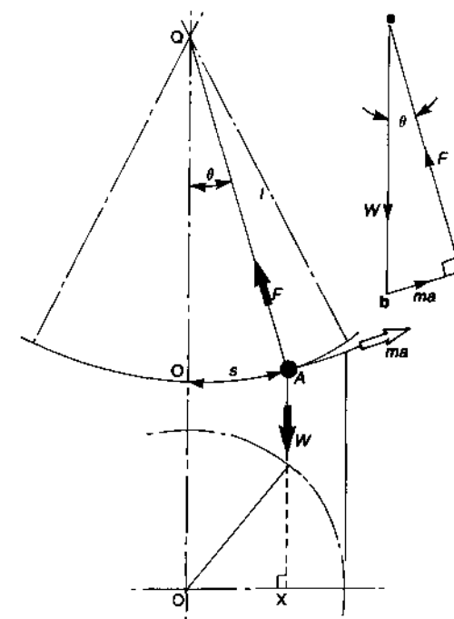
Fig. 8.14 Simple pendulum
