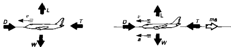
(a) Steady, level flight
